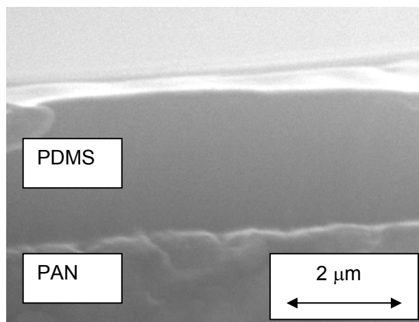
Figure 1: Freeze fractured membrane cross-section showing a nominal 2 \mu\text{m} PDMS layer on the PAN (Polyacrylonitrile) substrate - measured layer thickness could vary between 1.5 and 3 \mu\text{m} for different membrane samples.
